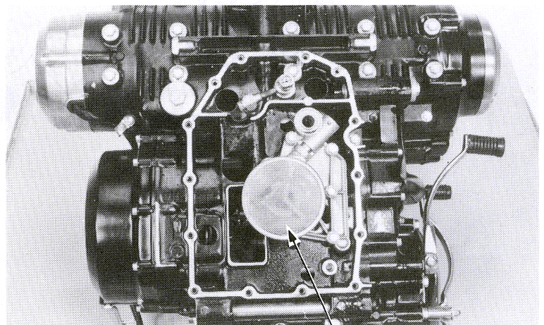
OIL STRAINER
